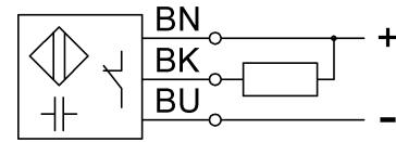
Wiring Diagram
